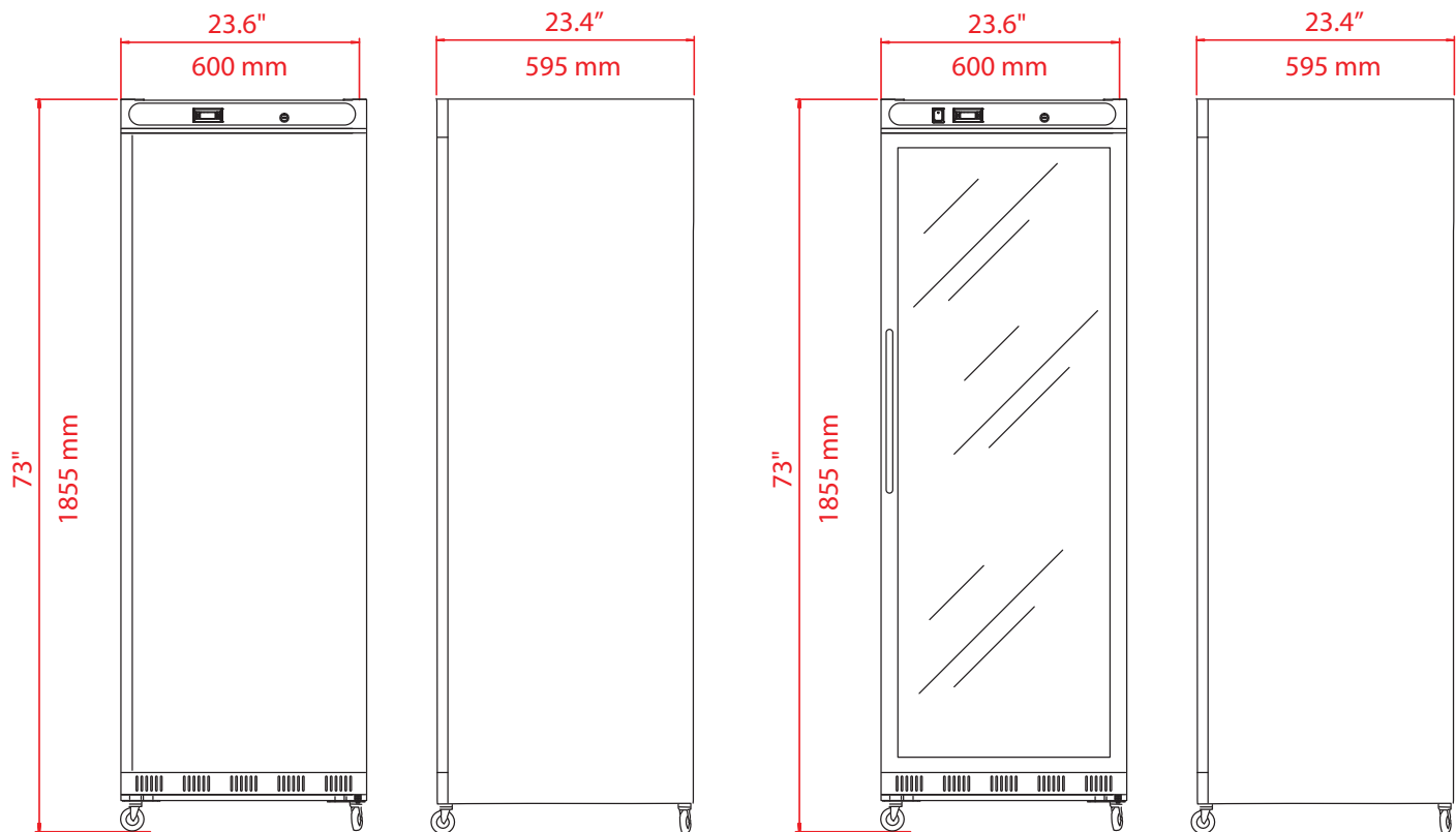
IB15R/IB15F
